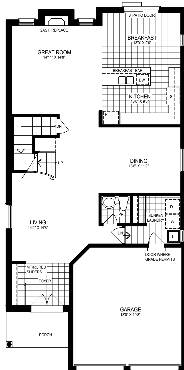
GROUND FLOOR PLAN ELEVATION 'B'
