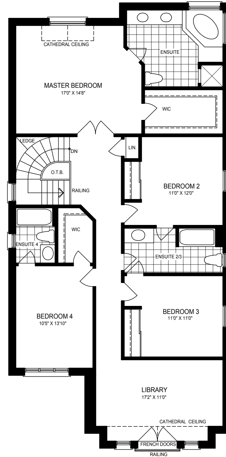
SECOND FLOOR PLAN ELEVATION 'B'
