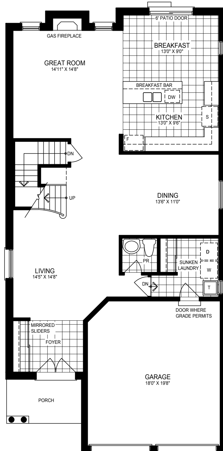
GROUND FLOOR PLAN ELEVATION 'C'
